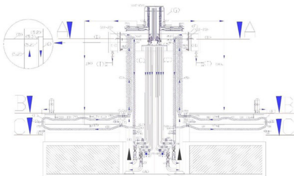
Figure 3: Vertical Desalinators-Demineralizers By Ion Exchange with Hydroelectric Energy Production. http://www.spawhe.eu
